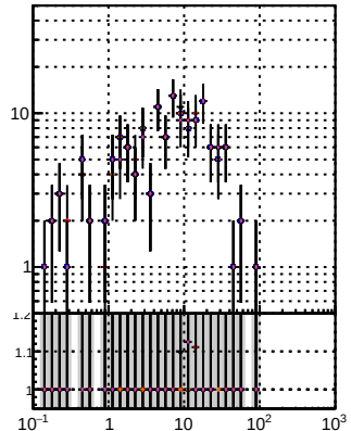
N of reco track vs \eta Orig/DQM orig MS DQM orig MS detached DQM orig MS
