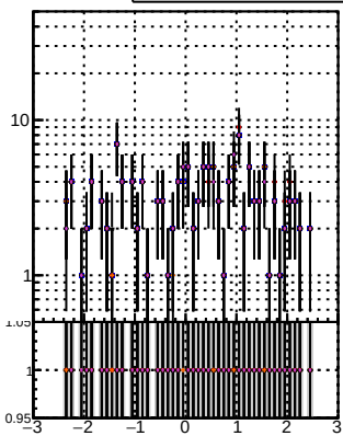
N of reco track vs \eta Orig/DQM orig MS DQM orig MS detached DQM orig MS
