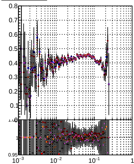
Fake rate vs dr Orig/DQM_orig_MS higher/DQM_orig_MS detached/DQM_orig_MS
