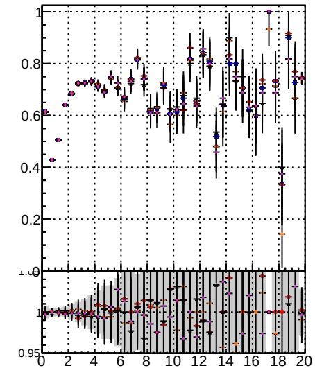
Orig/DQM_orig_MS Pileup/DQM_orig_MS Detached/DQM_orig_MS Fake rate vs.
