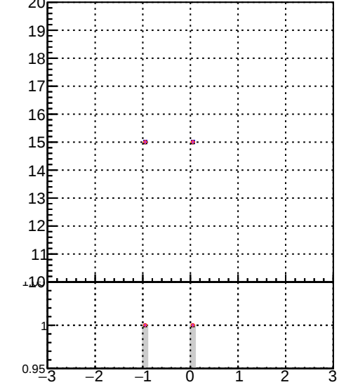
mean hit 0.00/DOM orig MS initial/DOM orig MS highPTtriple/DOM orig MS detached/DOM orig MS detachedT/DOM orig MS
