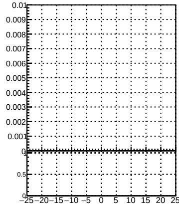
Duplicates Rate vs Dxy(PV)
