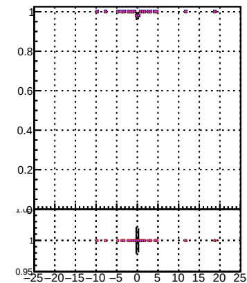
Fake rate vs d Legend: Original/DOM orig MS Initial/DOM orig MS High Pileup/DOM orig MS Detached/DOM orig MS
