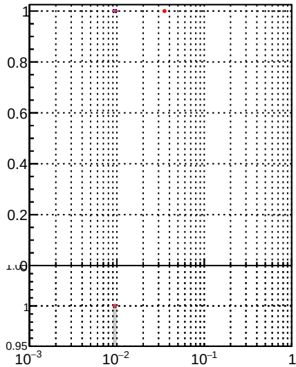
Fake rate vs \frac{\text{Orig/DQM\_orig\_MS}}{\text{higher/DQM\_orig\_MS}}
