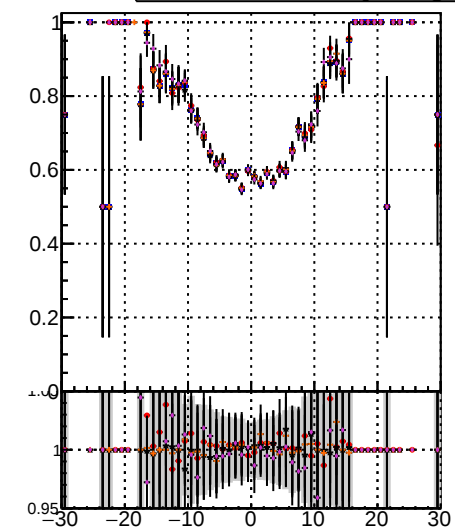
Orig/DQM_orig_MS higher/DQM_orig_MS detached/DQM_orig_MS Fake rate vs vertpos
