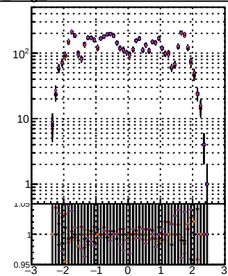
N of reco track vs \eta Orig/DQM-orig-MS dup/DQM-orig-MS detached/DQM-orig-MS
