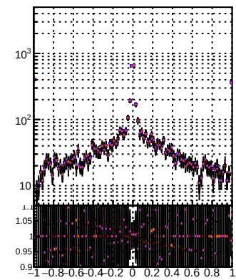
Orig/DOM orig MS detached O/DOM orig MS N of reco track vs d
