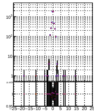
Orig/DOM orig MS detached O/DOM orig MS N of reco track vs d
