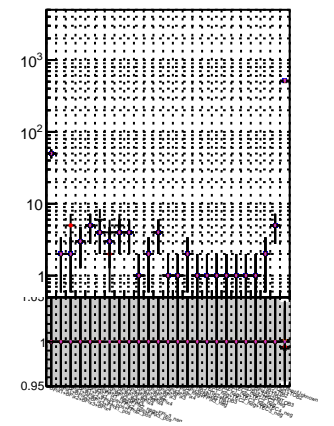
N of reco track vs. \chi^2 for different categories
