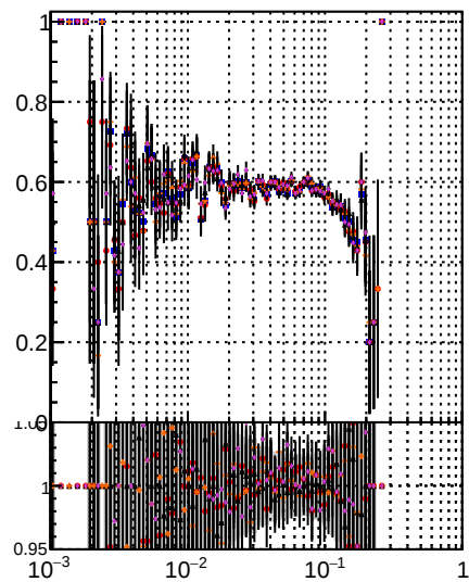
Fake rate vs \sqrt{s} Orig/DQM_orig_MS higher/DQM_orig_MS detached/DQM_orig_MS detached/DQM_orig_MS
