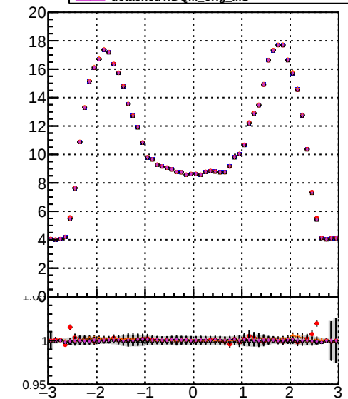
mean hit orig/DOM orig MS initial/DOM orig MS highPTtriple/DOM orig MS detachedO/DOM orig MS detachedT/DOM orig MS
