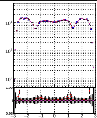
N of reco track vs \eta Orig/DQM_orig_MS multi/DQM_multi_MS detached/DQM_detached_MS
