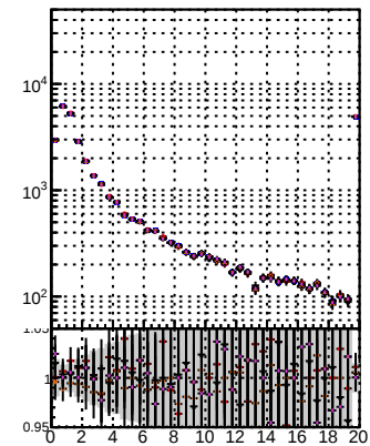
N of reco track vs. \chi^2 for different MS settings
