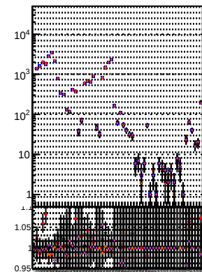
N of reco track vs. \chi^2 for different MS settings
