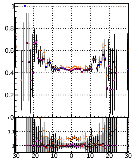
Orig/DQM_orig_MS higher/DQM_orig_MS detached/DQM_orig_MS Fake rate vs
