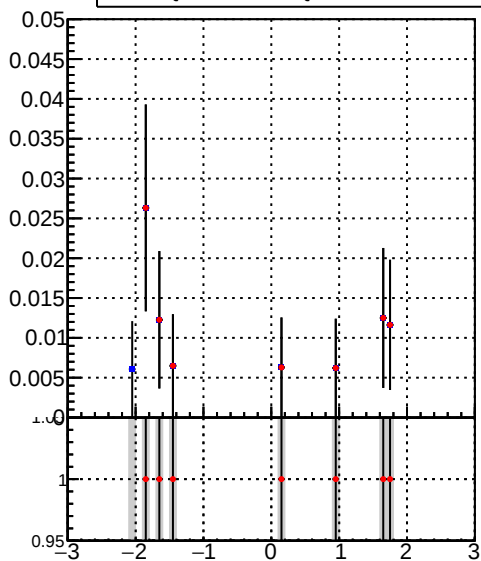
—•— /data2/legianni/BDT-vs-DNN/real-BDT/CMSSW_13_0_0_pre4/src/DQM_mkFit_time —•— DQM_TT__mkFit-DQM_time_mod
