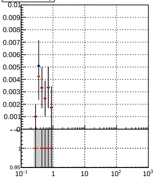
—•— /data2/legianni/BDT-vs-DNN/real-BDT/CMSSW_13_0_0_pre4/src/DQM_mkFit_time —•— DQM_TT__mkFit-DQM_time_mod
