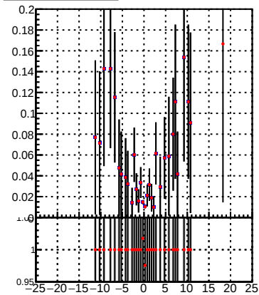
Efficiency vs Dxy(PV) - DQM TT_mkFit-DQM_time_mod
