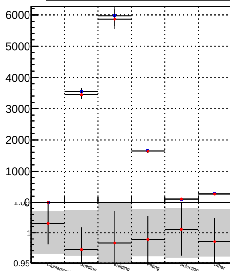
Average —●— DQM_TT_mkFit-DQM_time_mod
