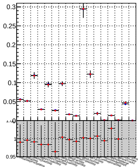
- /data2/legianni/BDT-vs-DNN/real-BDT/CMSSW_13_0_0_pre4/src/DQM_mkFit_time
