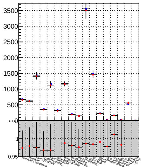
- /data2/legianni/BDT-vs-DNN/real-BDT/CMSSW_13_0_0_pre4/src/DQM_mkFit_time
