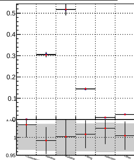
- /data2/legianni/BDT-vs-DNN/real-BDT/CMSSW_13_0_0_pre4/src/DQM_mkFit_time
