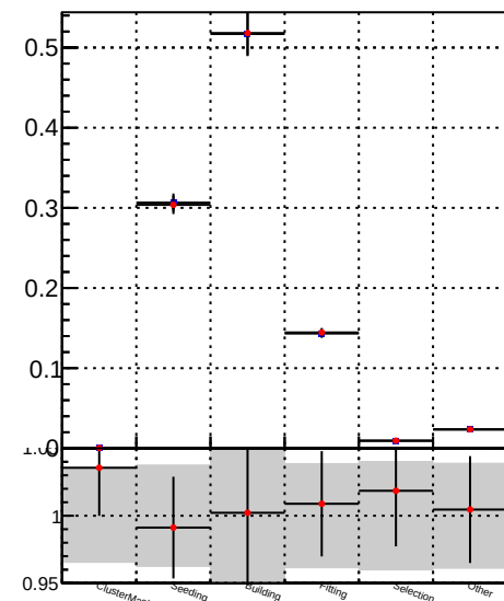
- /data2/legianni/BDT-vs-DNN/real-BDT/CMSSW_13_0_0_pre4/src/DQM_mkFit_time
