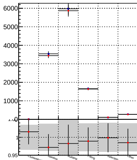
Average —●— DQM_TT__mkFit-DQM_time_mod
