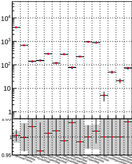
Number —●— DQM_TT_mkFit-DQM_time_mod
