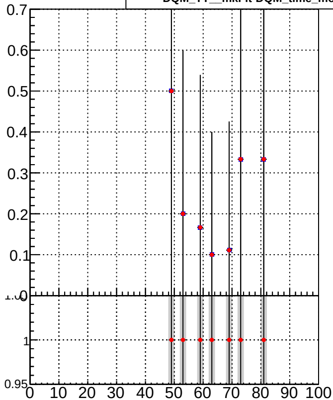
■ /data2/legianni/BDT-vs-DNN/real-BDT/CMSSW_13_0_0_pre4/src/DQM_mkFit_time ● DQM_TT_mkFit-DQM_time_mod
