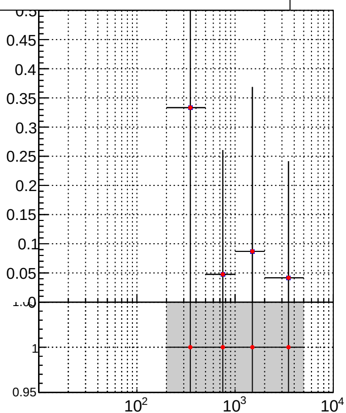
■ /data2/legianni/BDT-vs-DNN/real-BDT/CMSSW_13_0_0_pre4/src/DQM_mkFit_time ● DQM_TT_mkFit-DQM_time_mod
