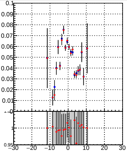
—■— /data2/legianni/BDT-vs-DNN/real-BDT/CMSSW_13_0_0_pre4/src/DQM_mkFit_time —●— DQM_TT_mkFit-DQM_time_mod
