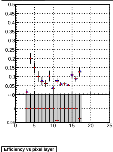
Efficiency vs pixel layer
