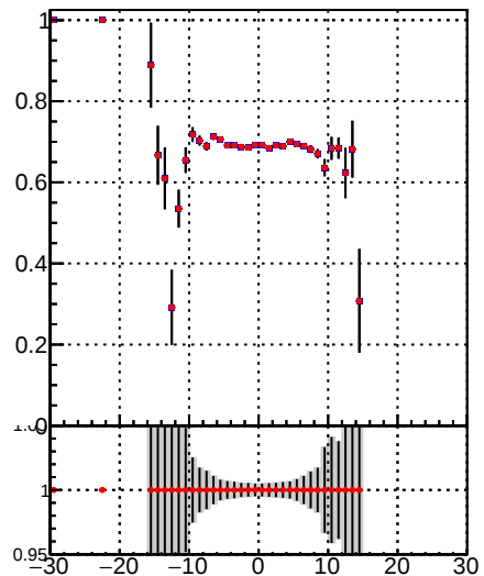
—•— /data2/legianni/BDT-vs-DNN/real-BDT/CMSSW_13_0_0_pre4/src/DQM_mkFit_time —•— DQM_TT_mkFit-DQM_time_mod
