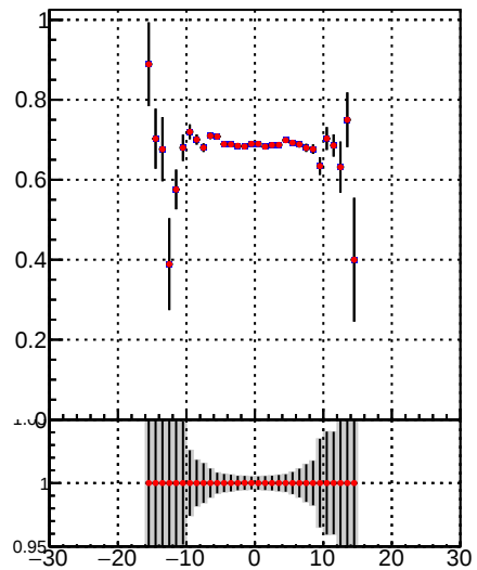
—•— /data2/legianni/BDT-vs-DNN/real-BDT/CMSSW_13_0_0_pre4/src/DQM_mkFit_time —•— DQM_TT_mkFit-DQM_time_mod
