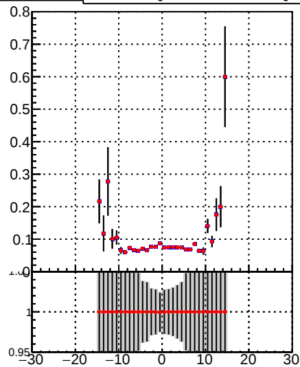
—•— /data2/legianni/BDT-vs-DNN/real-BDT/CMSSW_13_0_0_pre4/src/DQM_mkFit_time —•— DQM_TT_mkFit-DQM_time_mod
