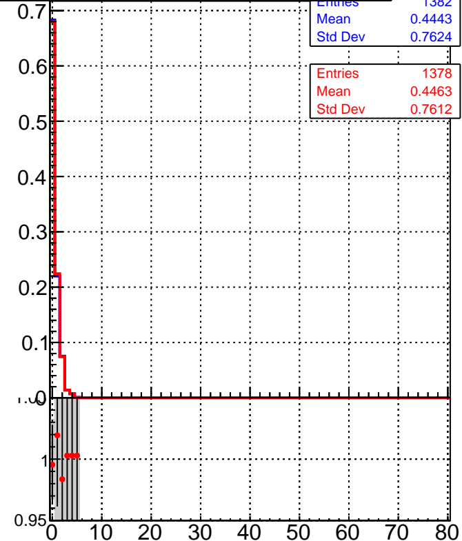
■ /data2/legianni/BDT-vs-DNN/real-BDT/CMSSW_13_0_0_pre4/src/DQM_mkFit_time ● DQM_TT_mkFit-DQM_time_mod
