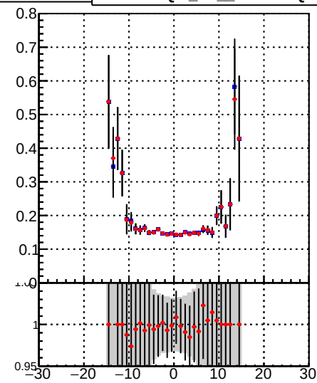
—•— /data2/legianni/BDT-vs-DNN/real-BDT/CMSSW_13_0_0_pre4/src/DQM_mkFit_time —•— DQM_TT_mkFit-DQM_time_mod
