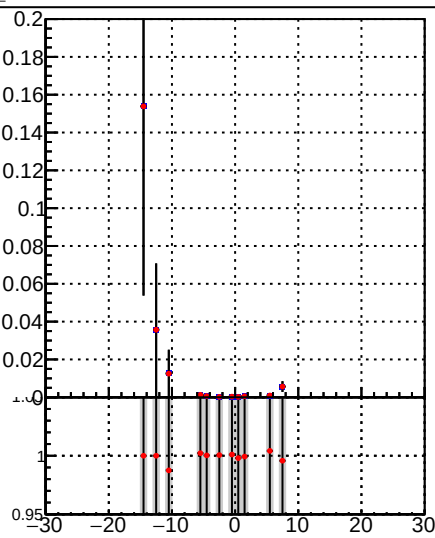
—•— /data2/legianni/BDT-vs-DNN/real-BDT/CMSSW_13_0_0_pre4/src/DQM_mkFit_time —•— DQM_TT_mkFit-DQM_time_mod
