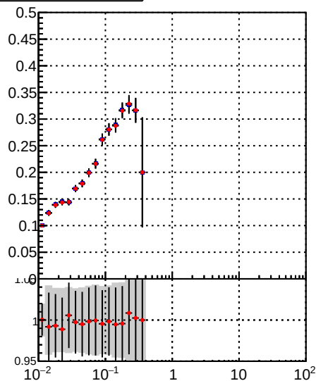
—•— /data2/legianni/BDT-vs-DNN/real-BDT/CMSSW_13_0_0_pre4/src/DQM_mkFit_time —•— DQM_TT_mkFit-DQM_time_mod
