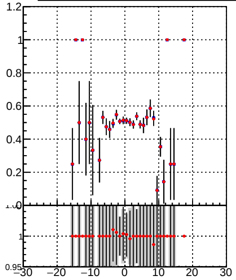
Efficiency vs. sim PV z — /data2/legianni/BDT-vs-DNN/real-BDT/CMSSW_13_0_0_pre4/src/DQM_mkFit_time — DQM_TT_mkFit-DQM_time_mod
