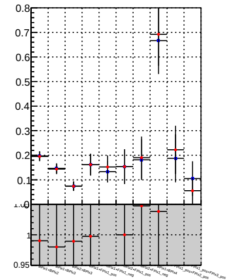
Fake rate vs. — /data2/legianni/BDT-vs-DNN/real-BDT/CMSSW_13_0_0_pre4/src/DQM_mkFit_time — DQM_TT_mkFit-DQM_time_mod
