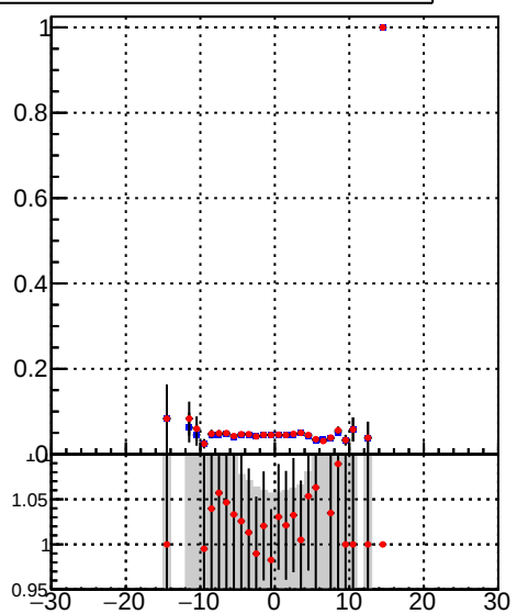
Efficiency vs vertpos - /data2/legianni/BDT-vs-DNN/real-BDT/CMSSW_13_0_0_pre4/src/DQM_mkFit_time - DQM_TT_mkFit-DQM_time_mod
