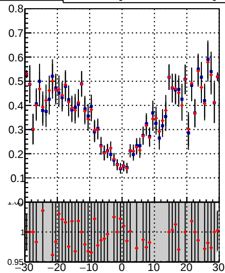
Legend: /data2/legianni/BDT-vs-DNN/real-BDT/CMSSW_13_0_0_pre4/src/DQM_mkFit_time (blue stars), DQM_TT_mkFit-DQM_time_mod (red stars)
