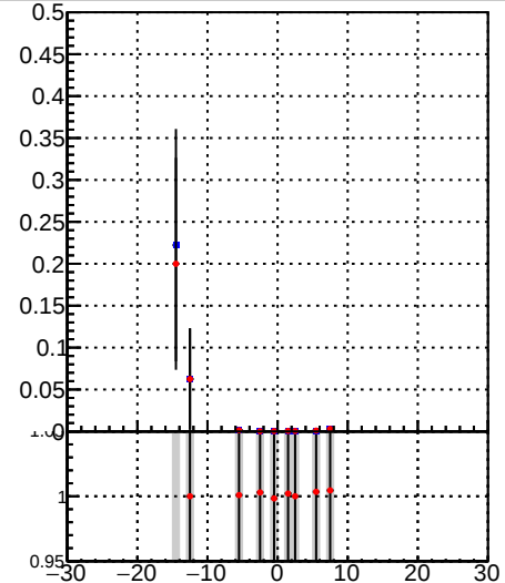
—•— /data2/legianni/BDT-vs-DNN/real-BDT/CMSSW_13_0_0_pre4/src/DQM_mkFit_time —•— DQM_TT_mkFit-DQM_time_mod
