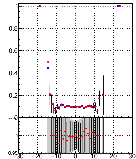
—•— /data2/legianni/BDT-vs-DNN/real-BDT/CMSSW_13_0_0_pre4/src/DQM_mkFit_time —•— DQM_TT_mkFit-DQM_time_mod
