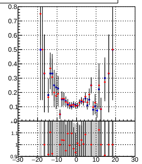
— /data2/legianni/BDT-vs-DNN/real-BDT/CMSSW_13_0_0_pre4/src/DQM_mkFit_time — DQM_TT_mkFit-DQM_time_mod
