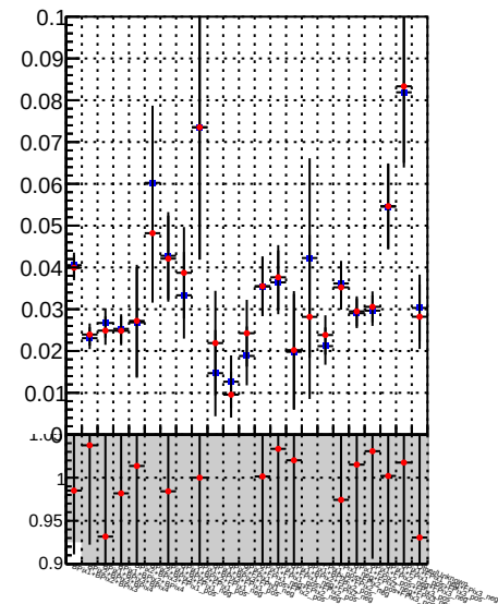
Fake rate vs. - /data2/legianni/BDT-vs-DNN/real-BDT/CMSSW_13_0_0_pre4/src/DQM_mkFit_time - DQM_TT_mkFit-DQM_time_mod
