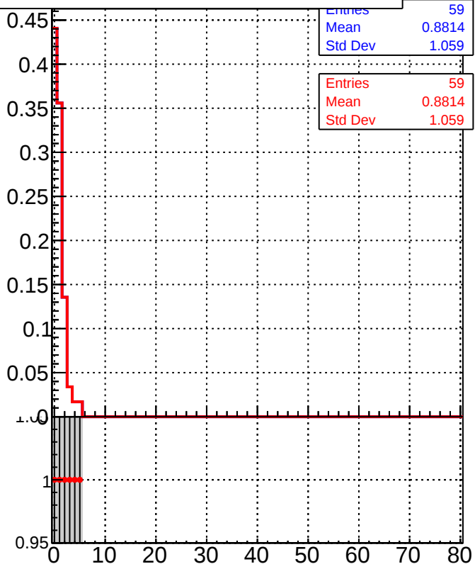
/data2/legianni/BDT-vs-DNN/real-BDT/CMSSW_13_0_0_pre4/src/DQM_mkFit_time DQM_TT_mkFit-DQM_time_mod
