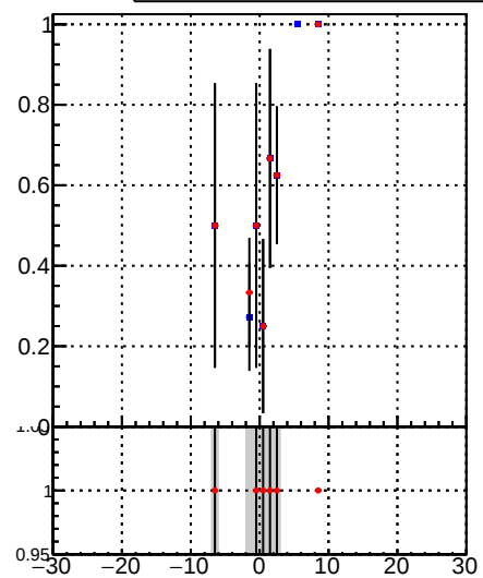
—■— /data2/legianni/BDT-vs-DNN/real-BDT/CMSSW_13_0_0_pre4/src/DQM_mkFit_time —●— DQM_TT_mkFit-DQM_time_mod
