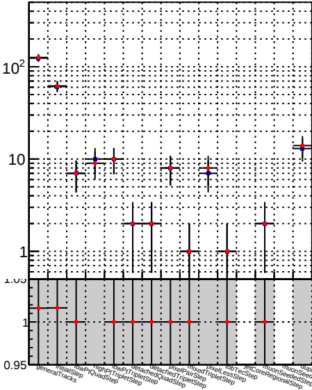
Number —●— DQM_TT__mkFit-DQM_time_mod
