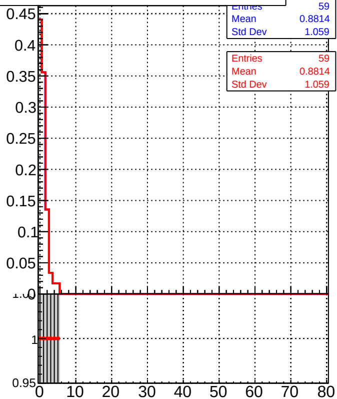
/data2/legianni/BDT-vs-DNN/real-BDT/CMSSW_13_0_0_pre4/src/DQM_mkFit_time DQM_TT_mkFit-DQM_time_mod
