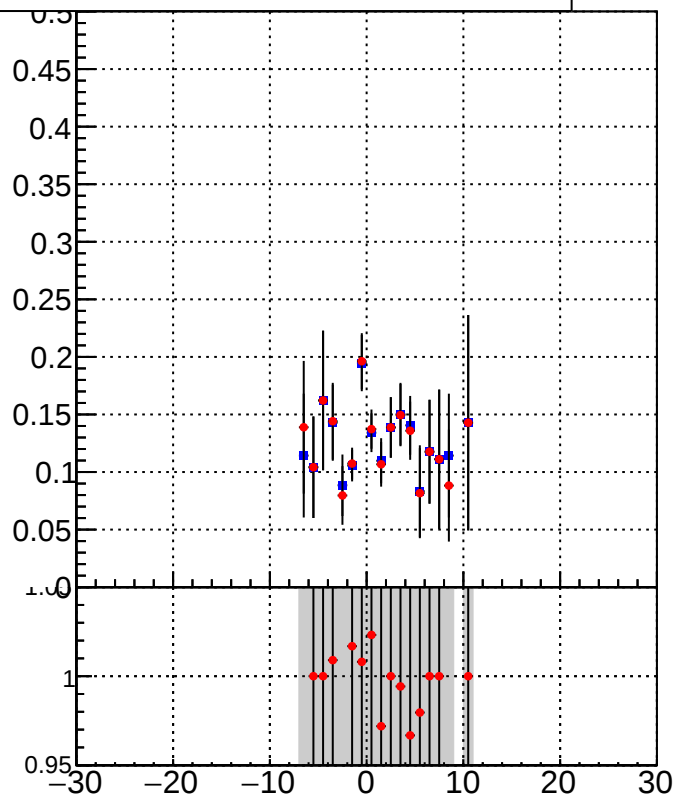
/data2/legianni/BDT-vs-DNN/real-BDT/CMSSW_13_0_0_pre4/src/DQM_mkFit_time DQM_TT__mkFit-DQM_time_mod
