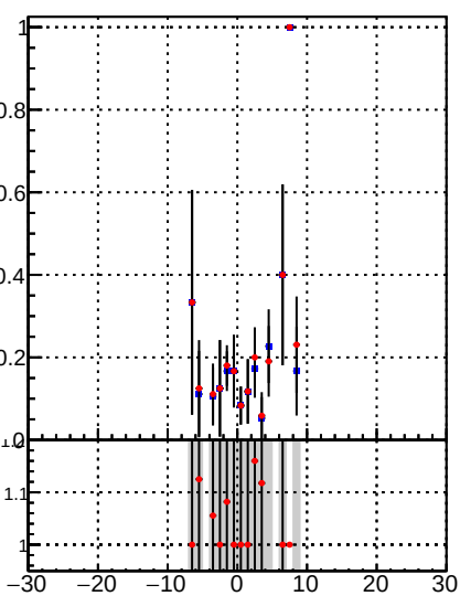
Fake rate vs d —●— /data2/legianni/BDT-vs-DNN/real-BDT/CMSSW_13_0_0_pre4/src/DQM_mkFit_time —●— DQM_TT_mkFit-DQM_time_mod
