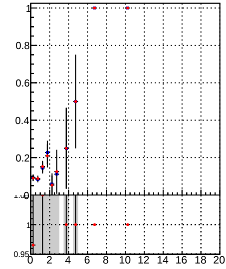
Fake rate vs. - /data2/legianni/BDT-vs-DNN/real-BDT/CMSSW_13_0_0_pre4/src/DQM_mkFit_time - DQM_TT_mkFit-DQM_time_mod
