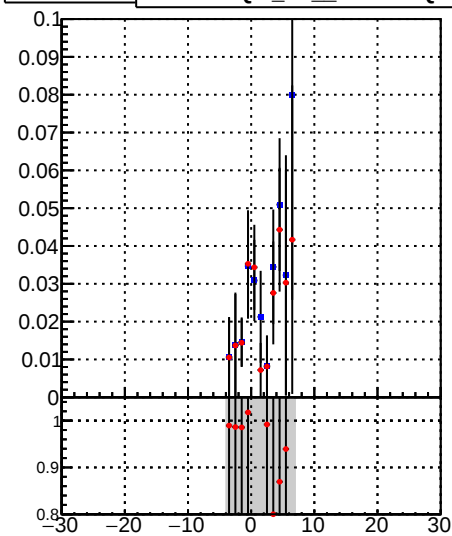
—•— /data2/legianni/BDT-vs-DNN/real-BDT/CMSSW_13_0_0_pre4/src/DQM_mkFit_time —•— DQM_TT_mkFit-DQM_time_mod
