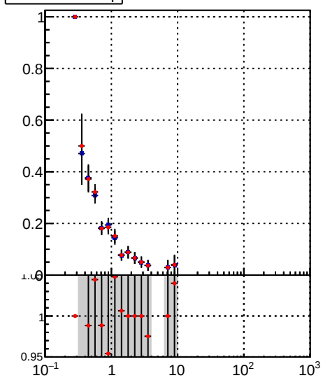
Pileup rate vs p_T
