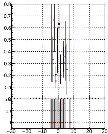
—●— /data2/legianni/BDT-vs-DNN/real-BDT/CMSSW_13_0_0_pre4/src/DQM_mkFit_time —●— DQM_TT_mkFit-DQM_time_mod
