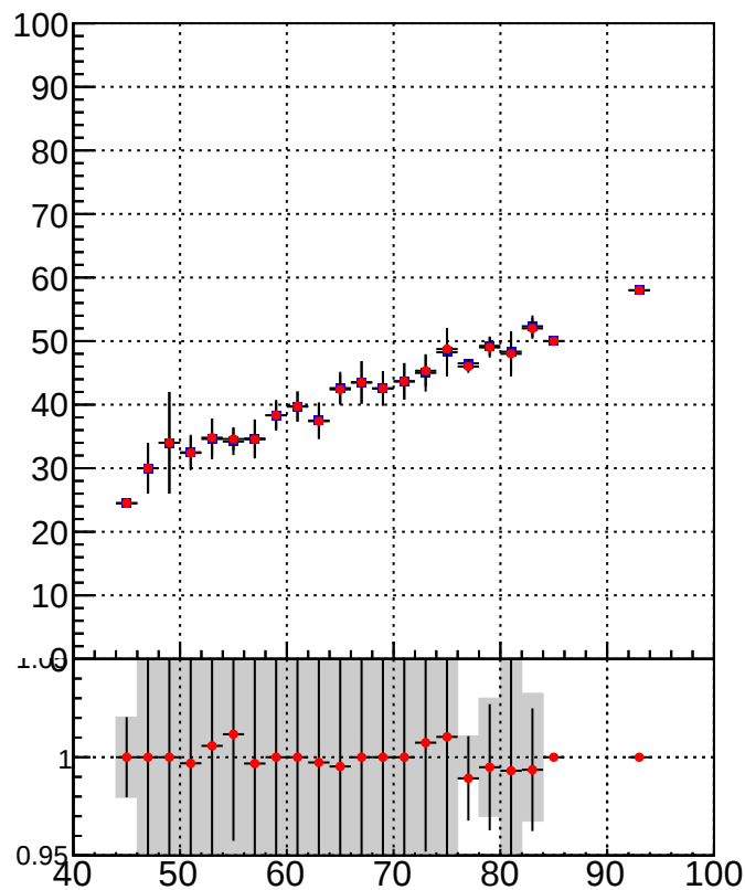
MatchedRecoVtx_vs_GenVtx
