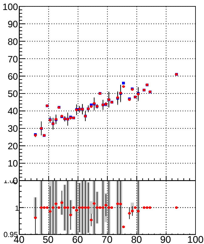
RecoVtx_vs_GenVtx
