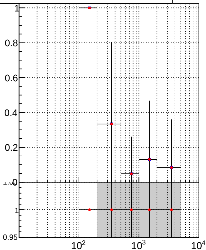
/data2/legianni/BDT-vs-DNN/real-BDT/CMSSW_13_0_0_pre4/src/DQM_mkFit_time DQM_TT_mkFit-DQM_time_mod
