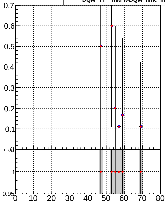
■ /data2/legianni/BDT-vs-DNN/real-BDT/CMSSW_13_0_0_pre4/src/DQM_mkFit_time ● DQM_TT_mkFit-DQM_time_mod
