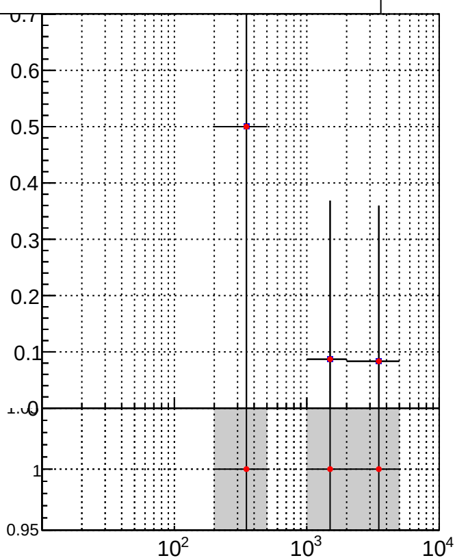
■ /data2/legianni/BDT-vs-DNN/real-BDT/CMSSW_13_0_0_pre4/src/DQM_mkFit_time ● DQM_TT_mkFit-DQM_time_mod
