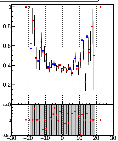
/data2/legianni/BDT-vs-DNN/real-BDT/CMSSW_13_0_0_pre4/src/DQM_mkFit_time
