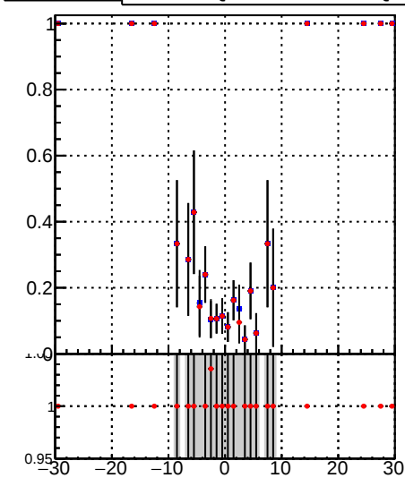
Legend: - \text{---} /data2/legianni/BDT-vs-DNN/real-BDT/CMSSW_13_0_0_pre4/src/DQM_mkFit_time - \text{---} DQM_TT_mkFit-DQM_time_mod
